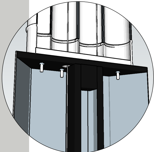
Connection Detail - Rigging Irons x2 and M10 Bolts x4 through both Mid and Base Section
