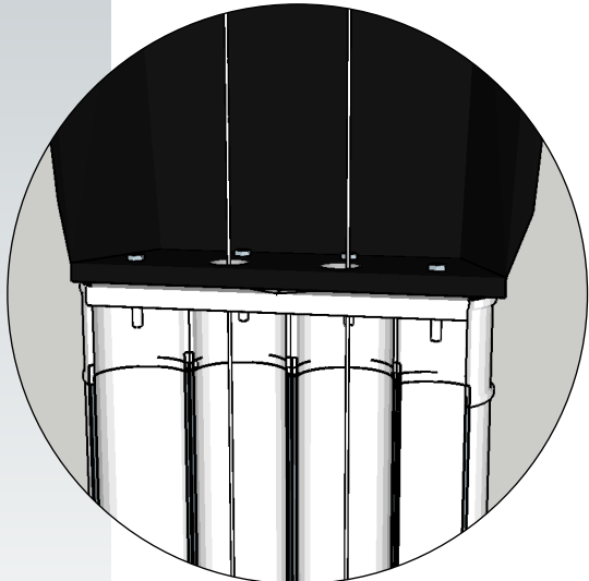
Connection Detail - Rigging Irons x2 and M10 Bolts x4 through both top and Mid Section
